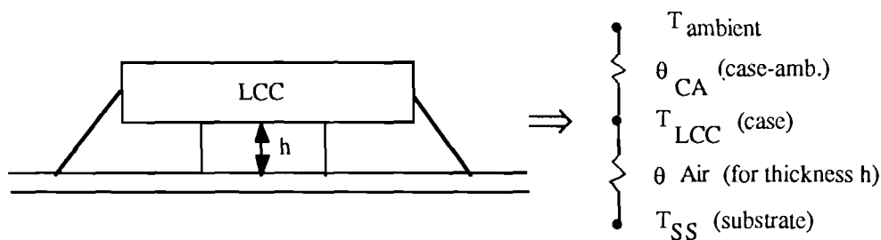
FIGURE 4.7-1: THERMAL MODEL
