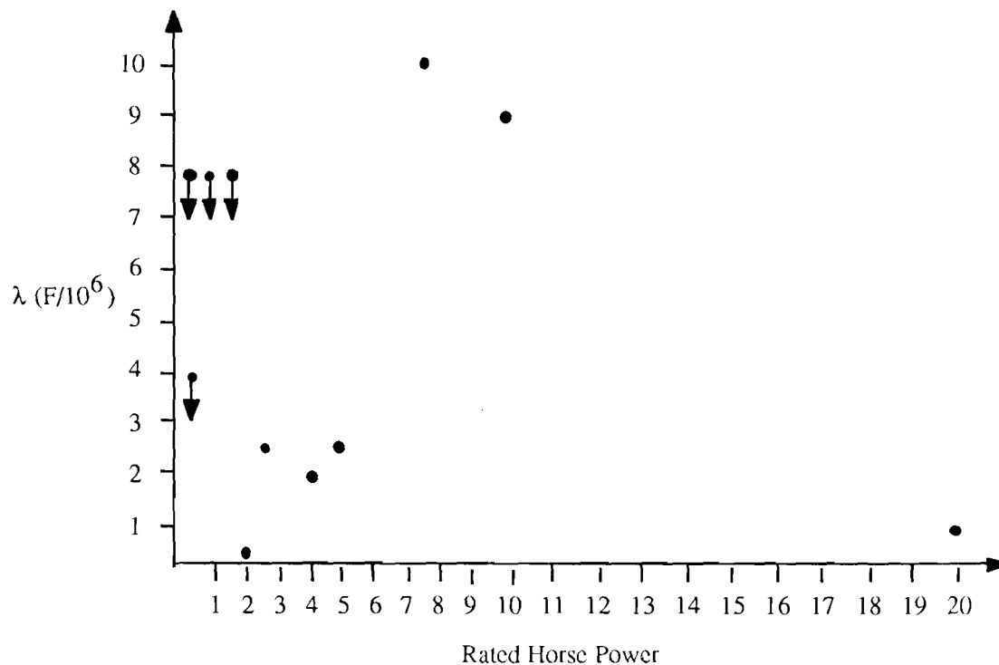
FIGURE 4.8-2: FAILURE RATES VS. HORSE POWER RATING
