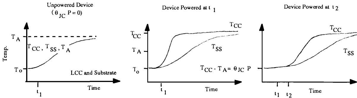
FIGURE 4.7-2: THERMAL PROFILE
