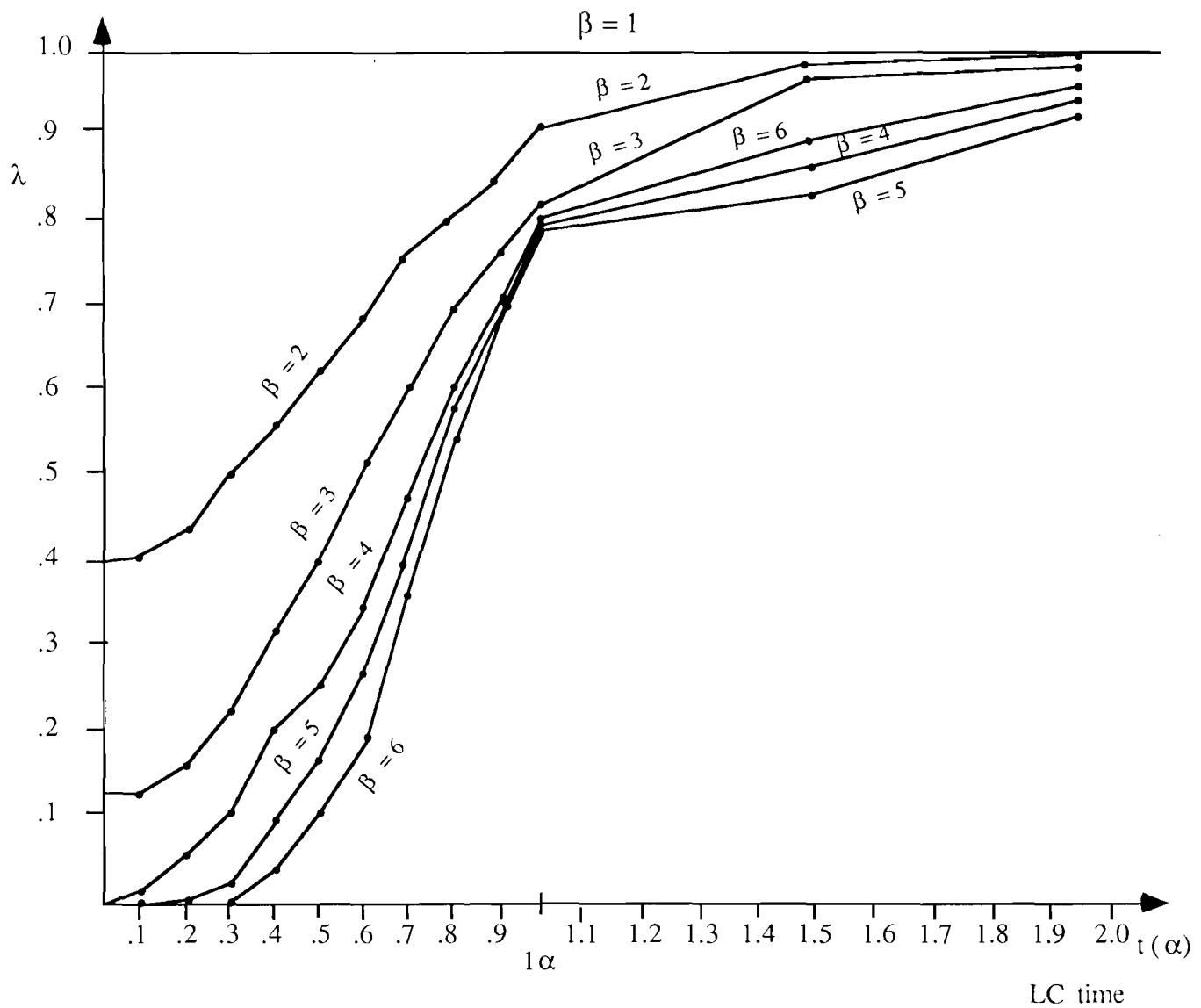
FIGURE 2.3-1: CUMULATIVE AVERAGE FAILURE RATE AS A FUNCTION OF LIFE CYCLE, \alpha , AND \beta
